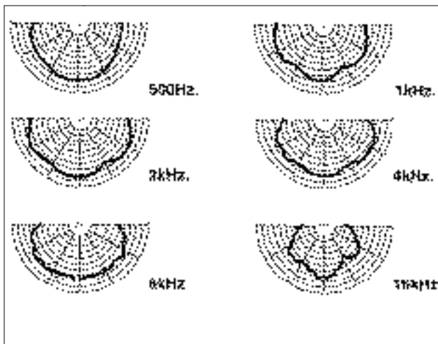
1 division = 5 dB
