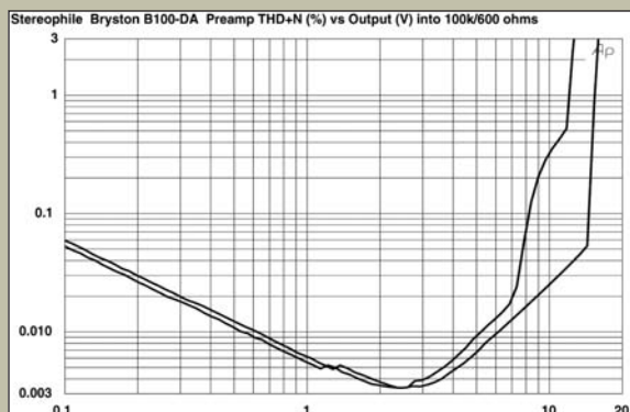
Fig.8 Bryston B100-DA, THD+noise (%) vs 1kHz output voltage into (from bottom to top): 100k, 600 ohms.
