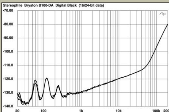
Fig.3 Bryston B100-DA, 1/2-octave spectrum with noise and spurs of digital black, 24-bit data (right channel dashed).
