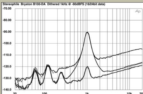
Fig.2 Bryston B100-DA, 1/2-octave spectrum with noise and spurs of dithered 1kHz tone at -90dBFS, 16-bit data (top) and 24-bit data (bottom). (Right channel dashed.)
