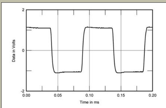
Fig.10 Bryston B100-DA, small-signal 10kHz squarewave into 8 ohms.
